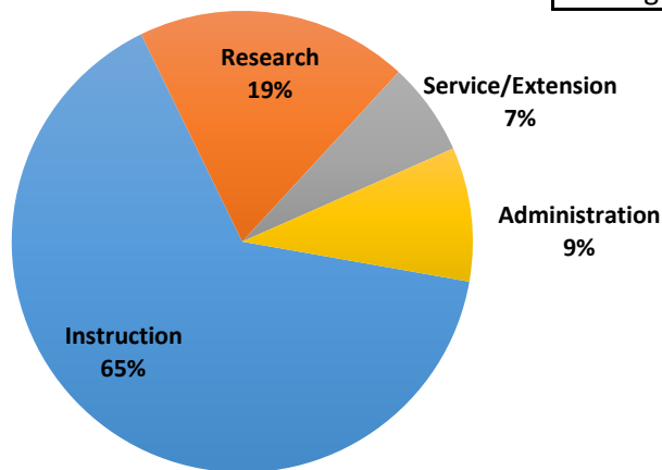
Average DOE
