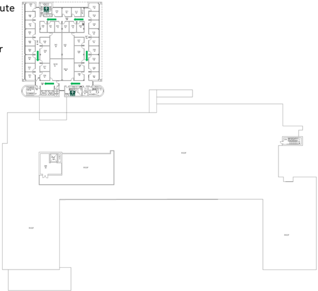
THIRD FLOOR PLAN CHARLES E. BARNHART BUILDING
